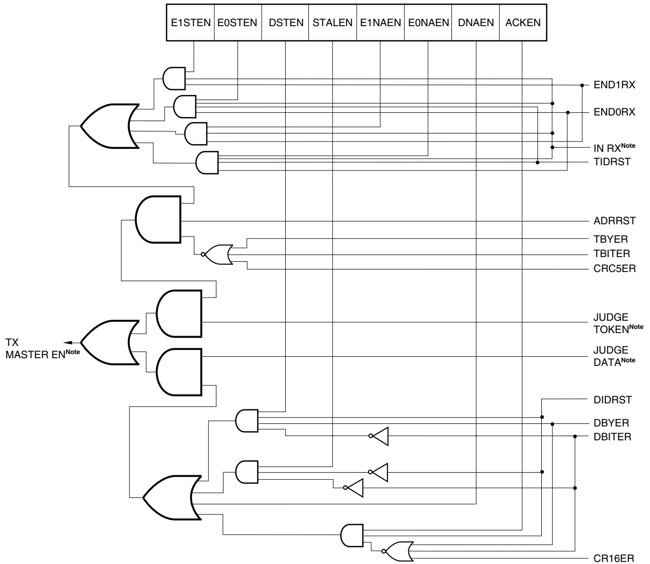
Figure 8-17. Configuration of Handshake Packet Transmit Reservation Register
