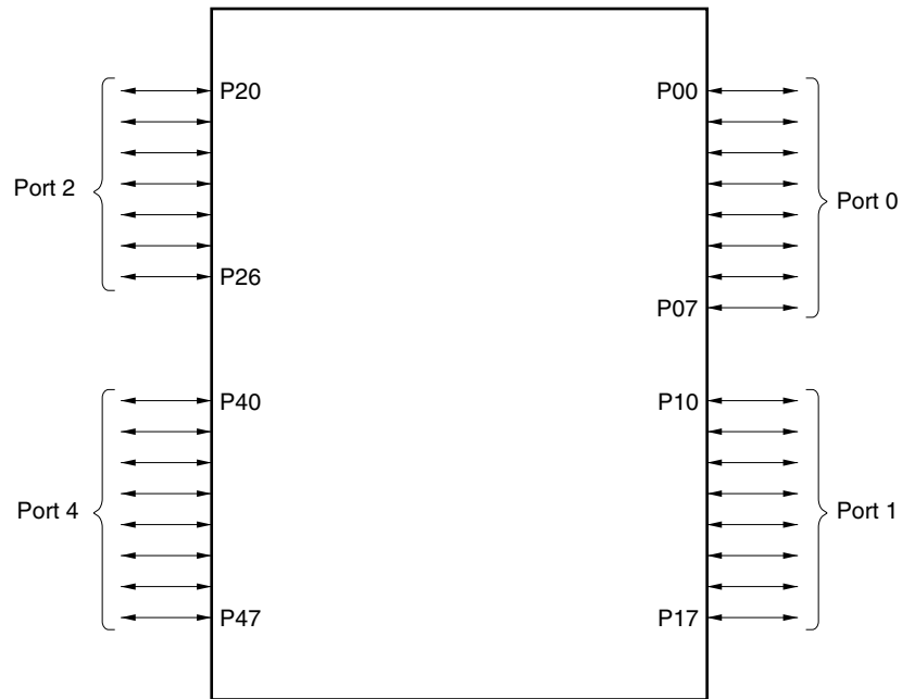
Figure 4-1. Port Types
