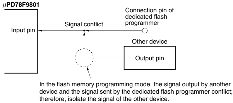
Figure 14-5. Signal Conflict (Input Pin of Serial Interface)
