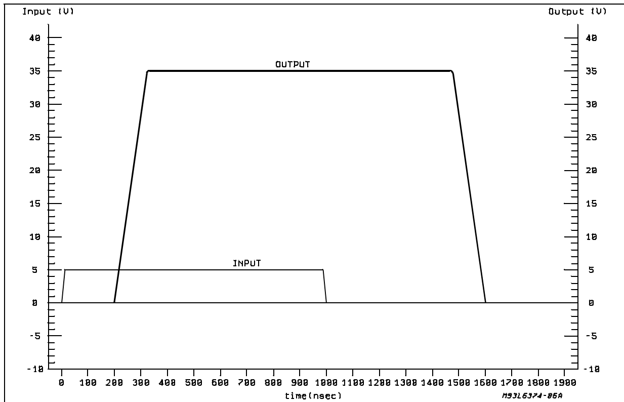
Figure 6. V_S = 35V , 350\Omega connected to V_S .
