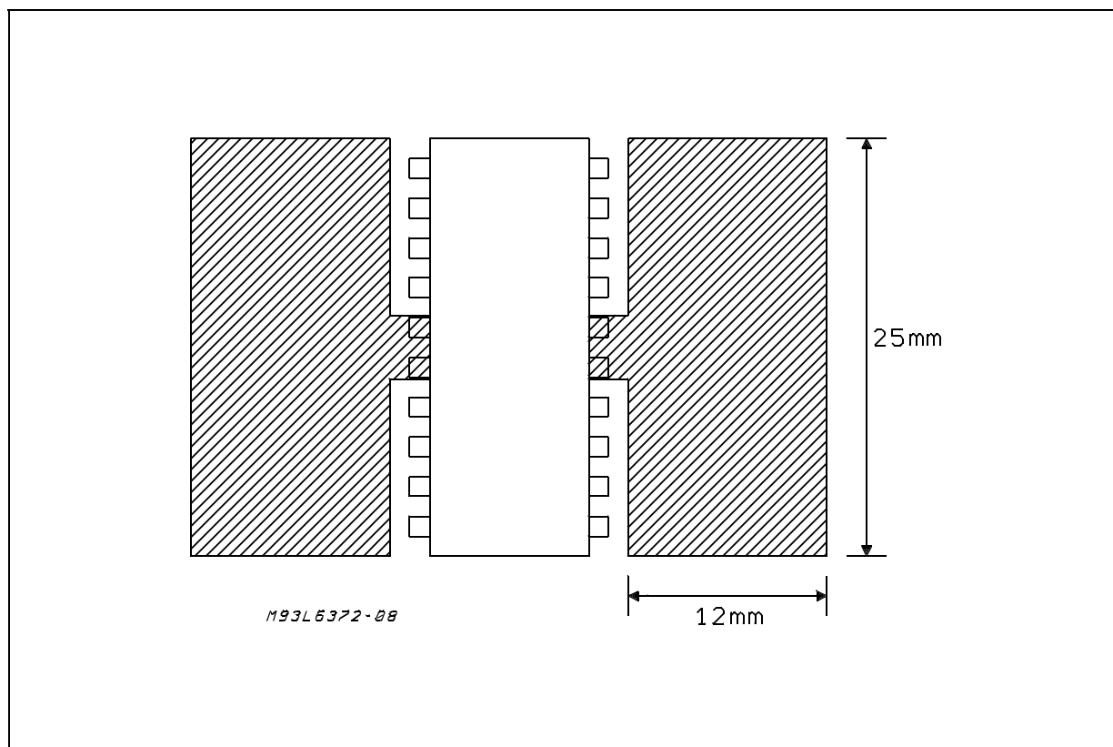
Figure 1: Printed Heatsink
