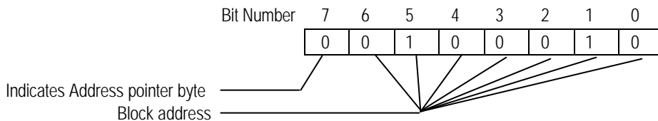
Figure 3. Example of an Address Pointer Byte
