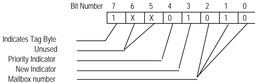
Figure 1. Example Tag Byte
