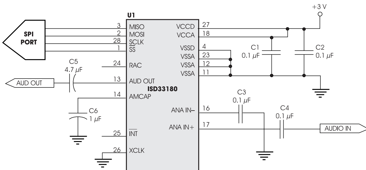
Figure 1: Circuit Example
