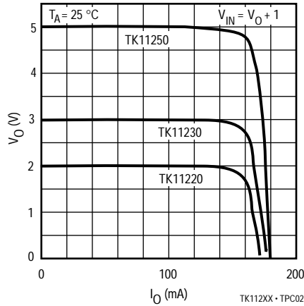
OUTPUT VOLTAGE vs. SHORT CIRCUIT CURRENT
