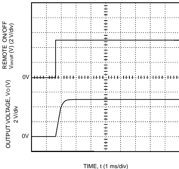
Figure 6. LC020A Typical Output Voltage Start-Up When Signal Applied to Remote On/Off
