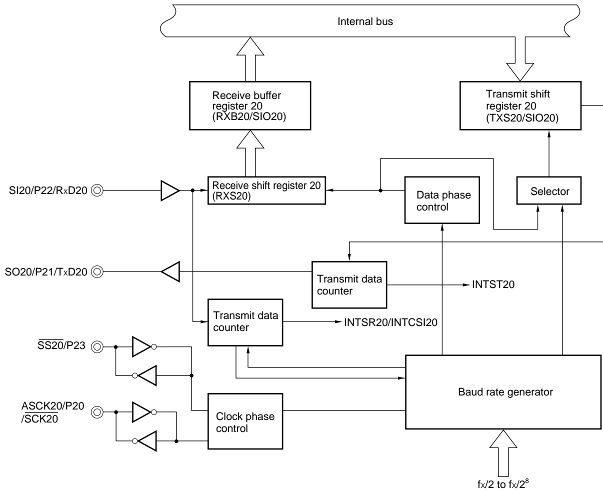
Figure 5-6. Serial Interface Block Diagram
