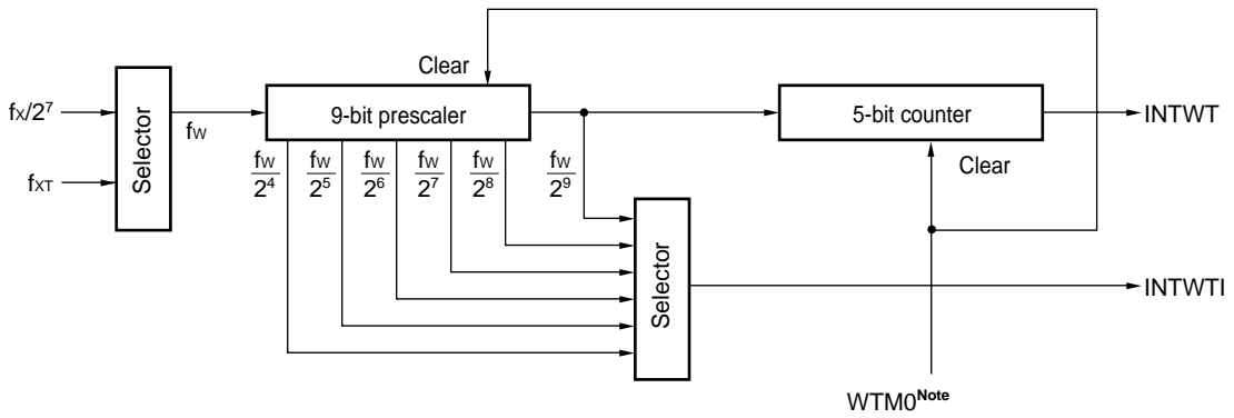
Figure 5-4. Watch Timer Block Diagram
