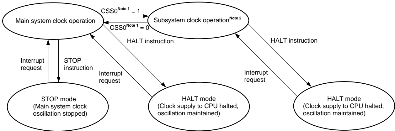
Figure 7-1. Standby Functions
