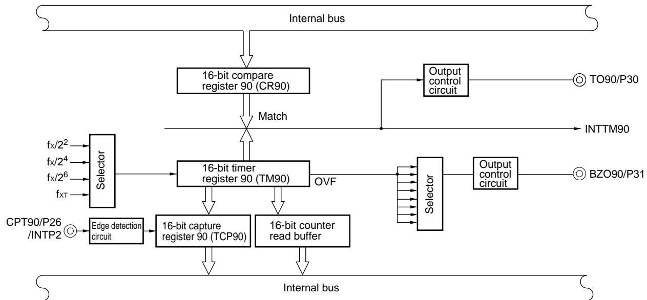
Figure 5-2. Block Diagram of 16-Bit Timer Counter 90
