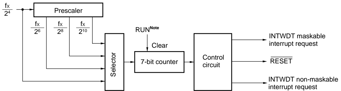
Figure 5-5. Watchdog Timer Block Diagram
