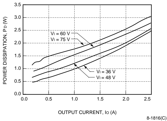
Figure 59. LW010F Typical Power Dissipation vs. Output Current at T_c = 25\text{ }^\circ\text{C}
