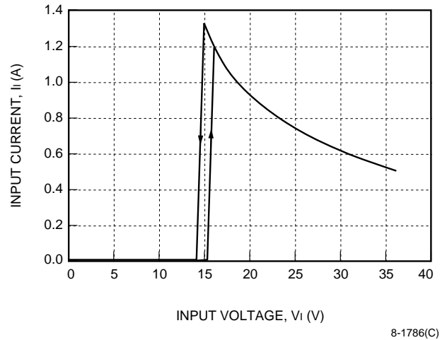
Figure 2. LC015 Input Current vs. Input Voltage at I_o = I_{o, max} and T_c = 25\text{ }^\circ\text{C}
