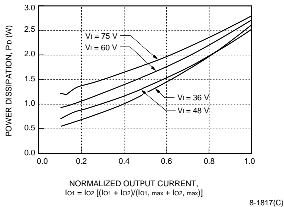
Figure 60. LW010AJ, BK, CL Typical Power Dissipation vs. Normalized Output Current at T_c = 25\text{ }^\circ\text{C}
