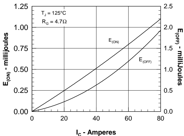
Fig. 7. Dependence of E_{ON} and E_{OFF} on I_C .
