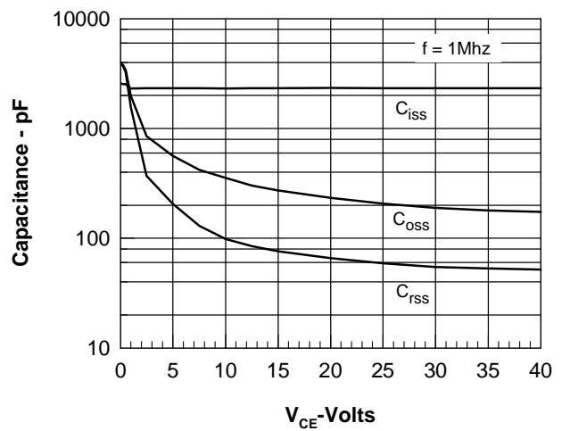
Fig. 6. Capacitance Curves
