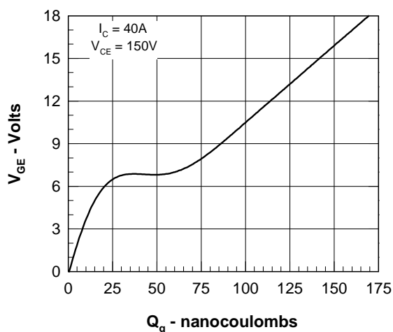
Fig. 9. Gate Charge
