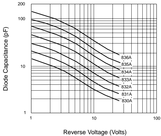
Diode Capacitance
